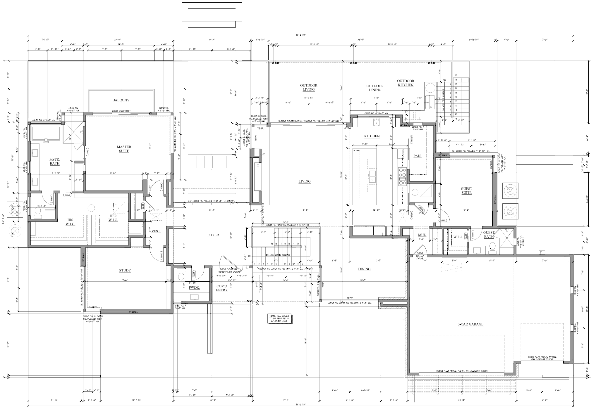
MAIN FLOOR DIMENSION PLAN SCALE 1/4" = 1'-0"
